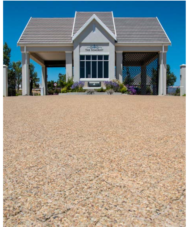
The Somerset Estate - 203 x 102mm Brownstone Coarse Exposed Aggregate pavers
